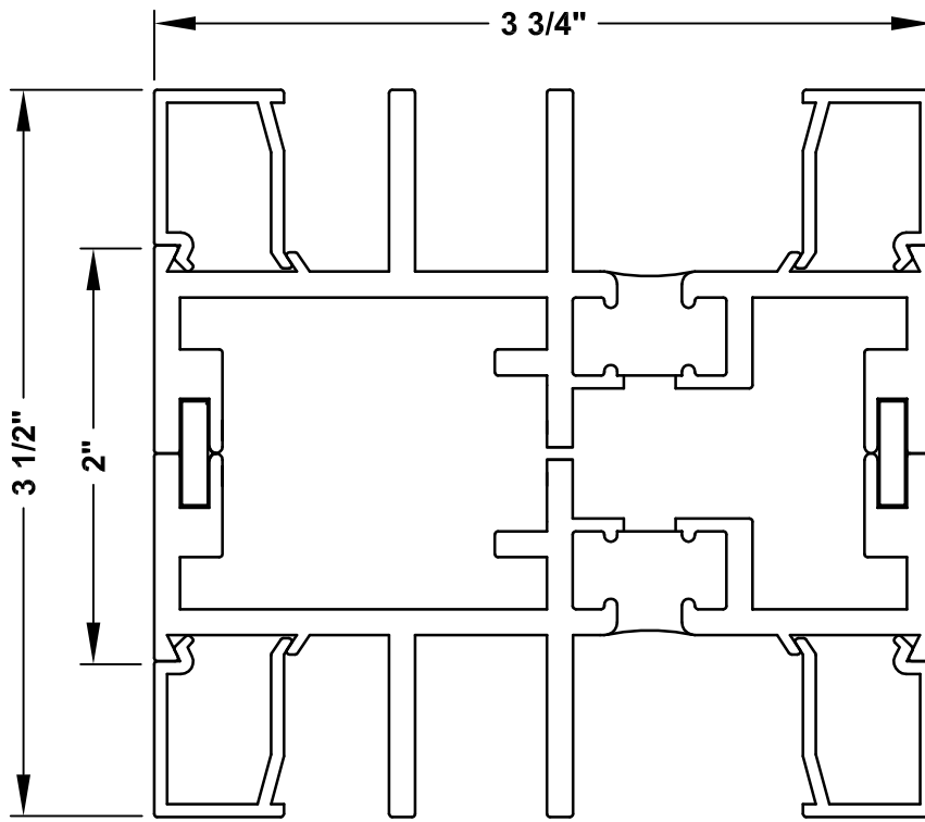
3750 BACK-TO-BACK MULLION
