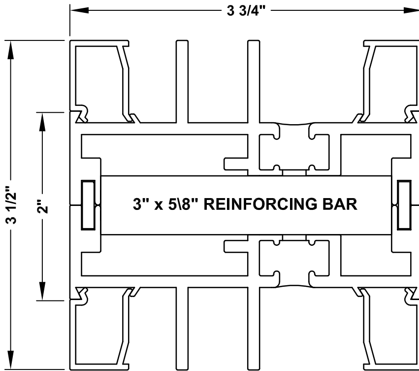
3750 BACK-TO-BACK MULLION WITH REINFORCING BAR
